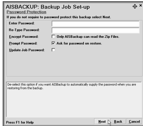
Figure 9: Password Protection.
