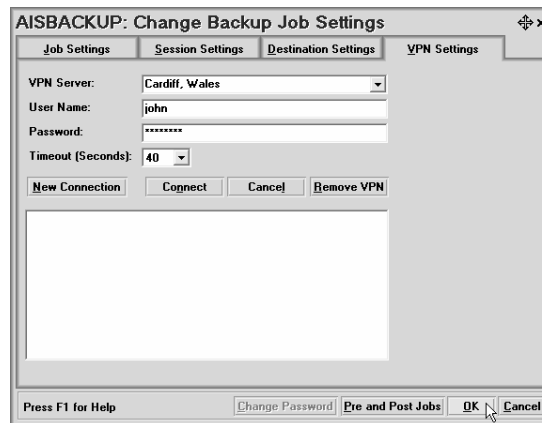
Figure 27: VPN Settings.
