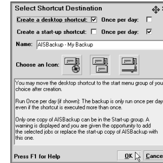
Figure 34: Create Shortcut.
