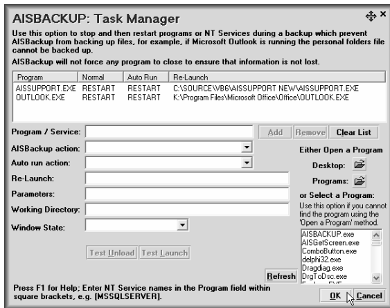
Figure 32: Task Manager.
