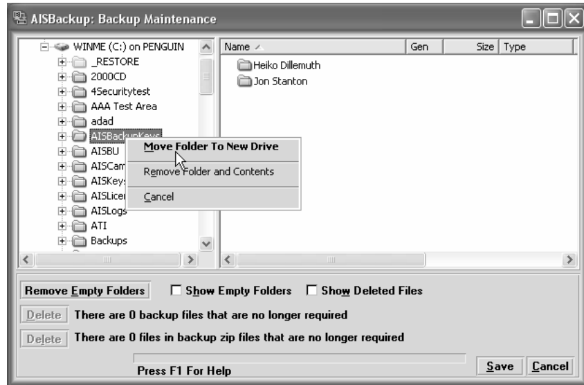
Figure 39: Backup Maintenance.
