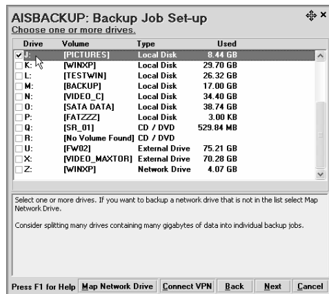
Figure 3: Select Drives.
