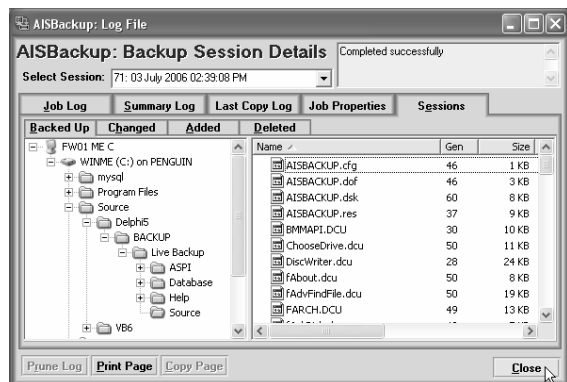
Figure 50: Sessions Log.
